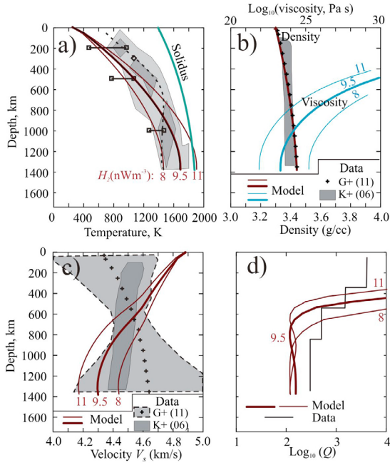
Figure 2. (a) Model lunar crust and mantle temperature structures using equation (8). Here fixed values are R_d = 1695 km (crustal thickness 45 km); R_c = 400 km; H_1 = 160 nWm ^{-3} and F_c = 0 . The effect of varying the mantle heating rate H_2 is shown; baseline model is in bold. The shaded regions show the probability distribution of the lunar temperature, from joint inversion of multiple data sets, replotted from Khan et al. [2006]. Squares joined by lines are from electromagnetic sounding [ Hood et al. , 1982]; diamond is from retention of mascon topography [ Lambeck and Pullan , 1980]. Dashed line is a convective model result from Zieth et al. [2009]. Green line is the peridotite solidus of Hirschmann [2000]. (b) Model mantle density (equation (9)) and viscosity structure. Density is compared with seismically-inferred values of Garcia et al. [2011] and Khan et al. [2006]. (c) Model S-wave velocity structure, evaluated at 1s, compared with Garcia et al. [2011] and Khan et al. [2006] values. (d) Model seismic Q at 1 s calculated using the approach outlined in section 3.1, assuming a grain-size of 1 cm and the baseline temperature profile shown in Figure 2a. For comparison the seismically-inferred Q summarized in Garcia et al. [2011] is shown.
