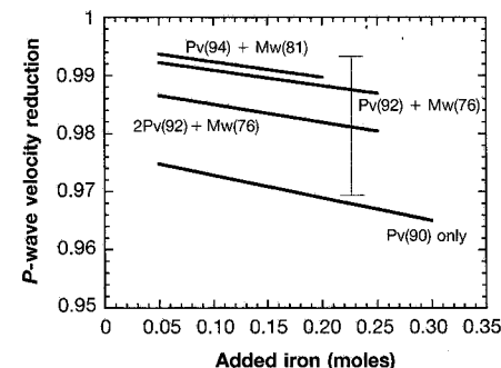
Fig. 4. Ratio of the P -wave velocity for assemblages that have undergone chemical reactions with variable amounts of Fe to that of the unreacted assemblage. The mole percent of Mg in perovskite (Pv) and magnesiowüstite (Mw) in the different unreacted assemblages are given in parentheses, and we derived the Fe/Mg ratios of these phases using the Fe-Mg partition coefficients of (22). The differing lengths of the lines is an indication of the maximum amount of Fe that can chemically react with the different assemblages, as given by Eq. 1. Because perovskite volumetrically dominates both the reacted and unreacted assemblages and no compositional dependence of the elastic properties (other than density) of perovskite has been observed (4, 5), the primary error in this ratio is produced by uncertainties in the elastic properties of FeO, FeSi, and SiO 2 ; the error bar reflects uncertainties in the bulk moduli and densities of these phases under CMB conditions.
