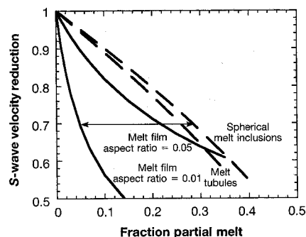
Fig. 3. The ratio of the S -wave velocity of melt-bearing mantle to that of solid mantle for varying melt fractions and melt geometries. The arrow corresponds to the variation in melt fraction implied by the inferred P -wave velocity depression of 10% coupled with the results in Fig. 2.
