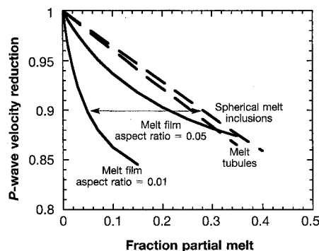
Fig. 2. The ratio of the P -wave velocity of melt-bearing mantle to that of solid mantle for varying melt fractions and melt geometries. The arrow indicates the range of melt fractions that produce a 10% P -wave velocity depression.
