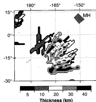
Fig. 1. Map view of the inferred thickness of the low-velocity anomaly, as constrained by SP diff /KS ray results. Because the energy of diffracted P waves along the CMB is constrained to lie predominantly in the lowermost 50 km of the mantle, the thickness of this feature may be estimated from a combination of the observed time of arrival and length of travel of this phase along the CMB and waveform analyses [(1)]. MH denotes the location of the anomaly characterized by Mori and Helmberger using precursors to the reflected PcP phase (2).
