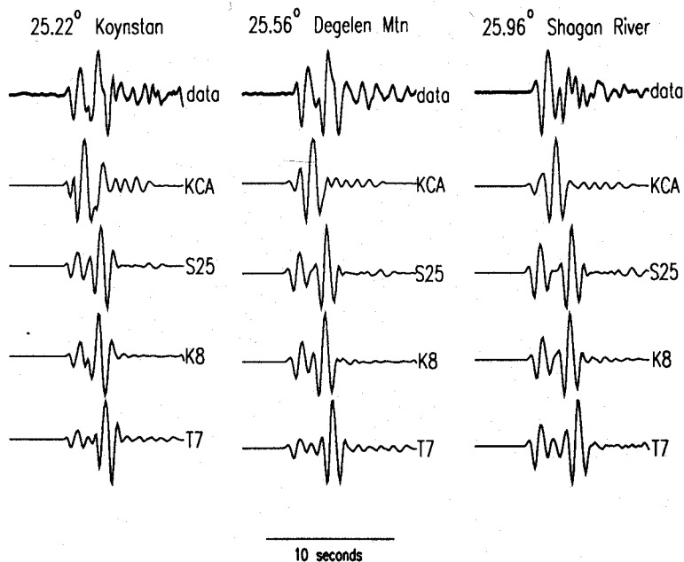
Figure 6. The three columns are separate stacks for events from the three Semipalatinsk sites recorded at station OBN (data are top trace, model predictions are bottom four traces). For these distances, the reflection off the 670 arrives around 2 or 3 s after the first arrival, and the 400 arrives outside the time window presented.
