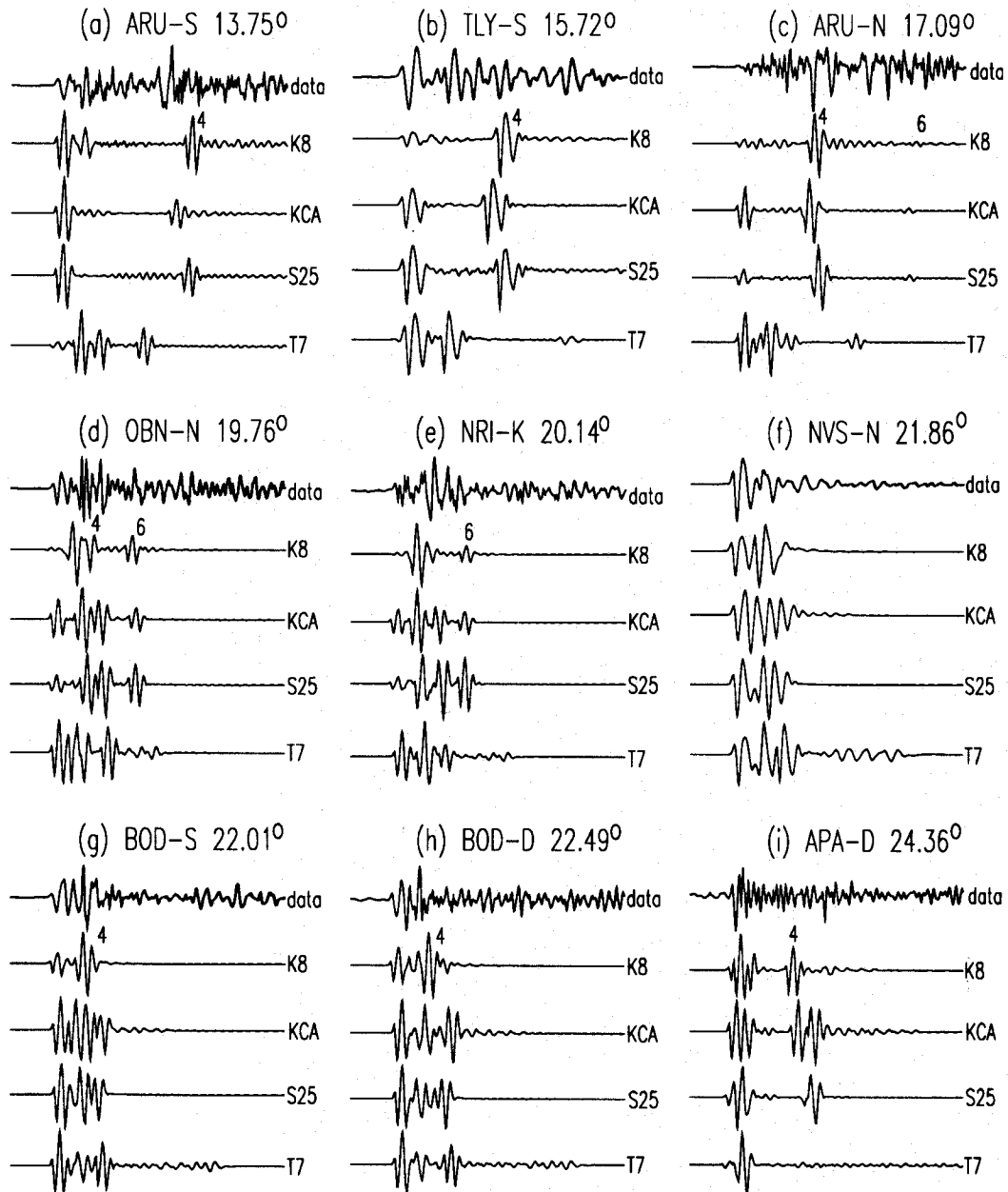
Figure 5. (a)–(i) present data stacks (top trace) and the predictions of the four models (bottom four traces.) The letter code next to the station names signifies the source location (D = Degelen Mountain, K = Koynstan, N = Novaya Zemlya, and S = Shagan River). Where the phases are well separated, the numbers '4' and '6' indicate arrivals from the 400 and 670 km discontinuities.
