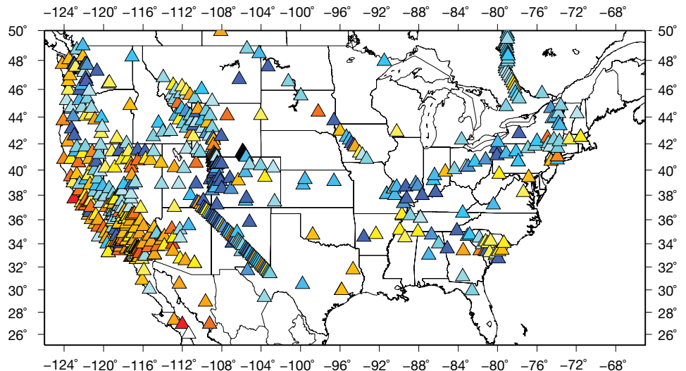
EARS automated crustal thickness estimates at almost 600 stations within the continental US.
